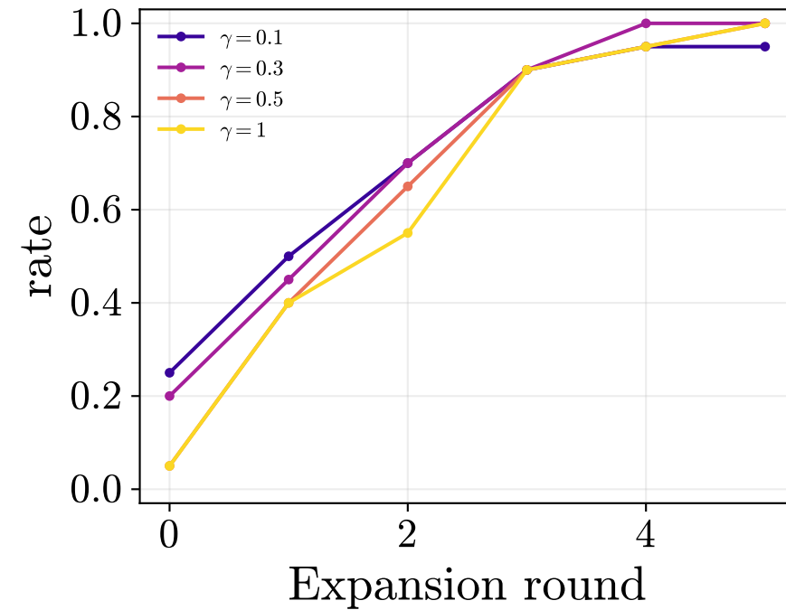
Raw success rate
