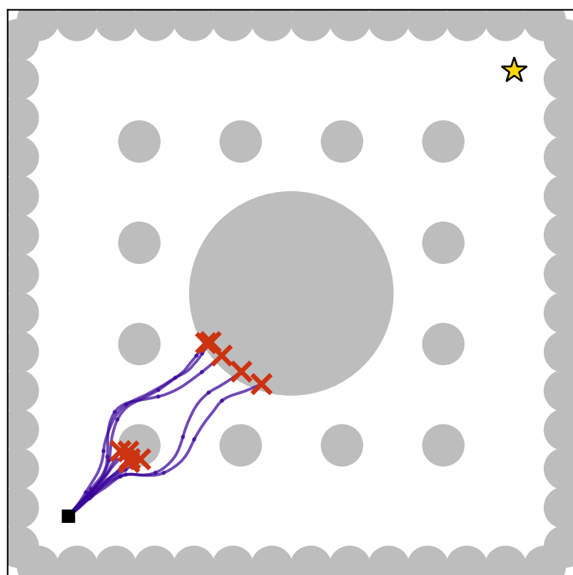
CFM-MPPI* w_s = 1.0
