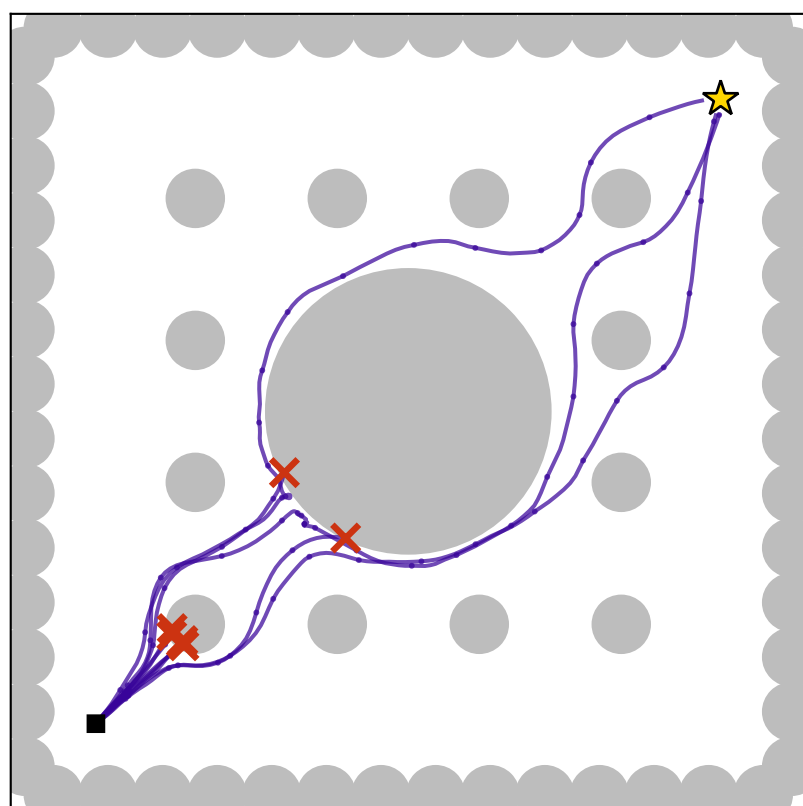
CFM-MPPI* w_s = 0.5
