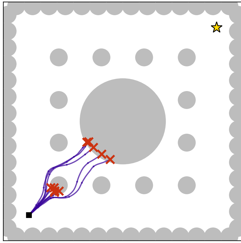
CFM-MPPI* w_s = 1.0
