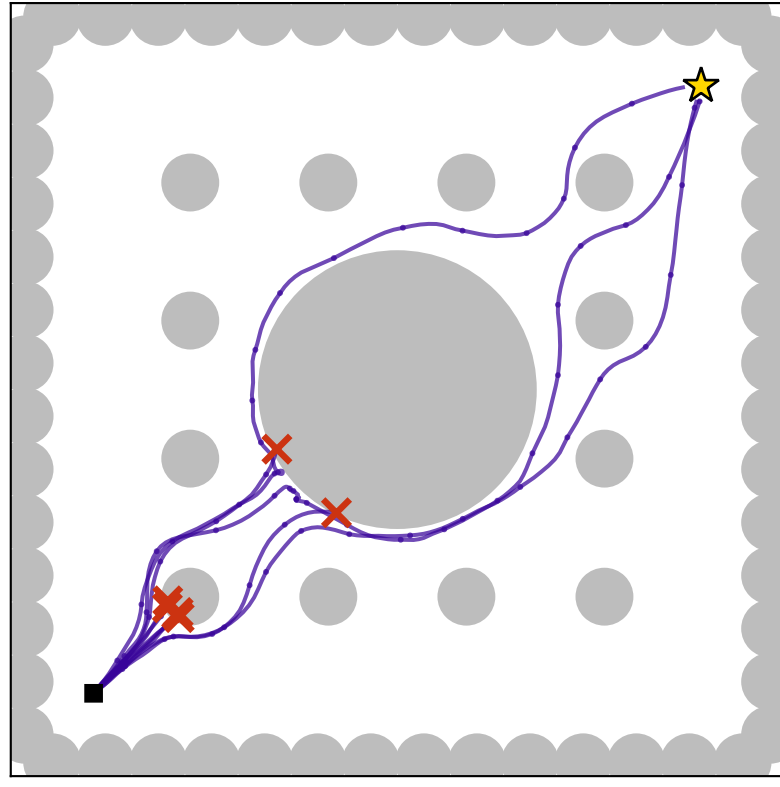
CFM-MPPI* w_s = 0.5
