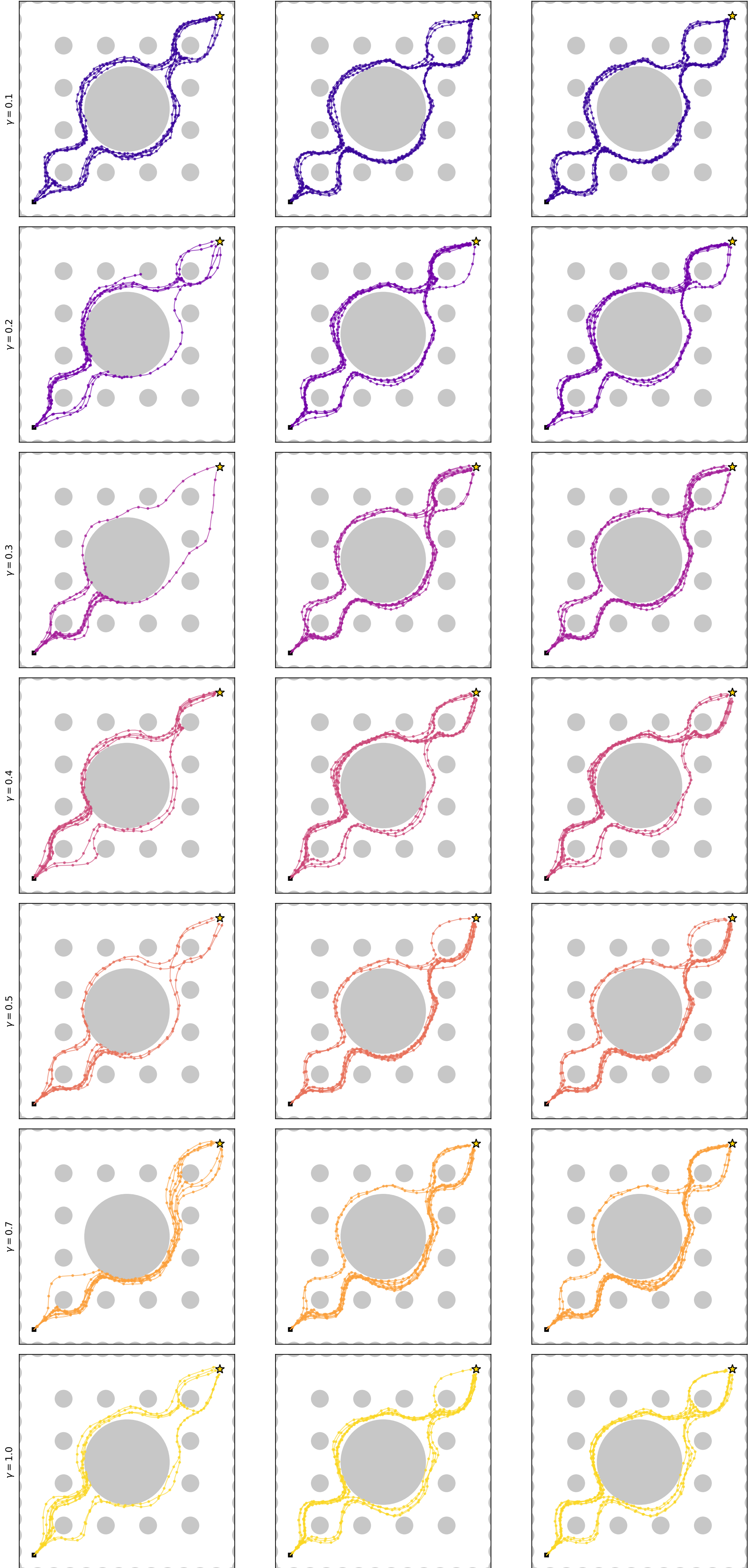
pretrained r0
