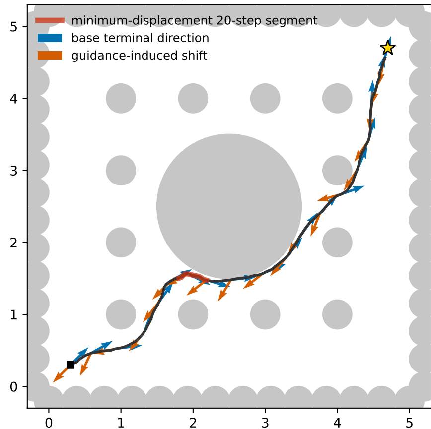
SR: task-space direction conflict
