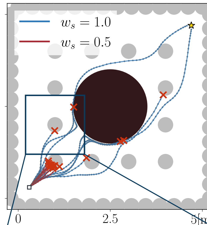
CFM-MPPI
