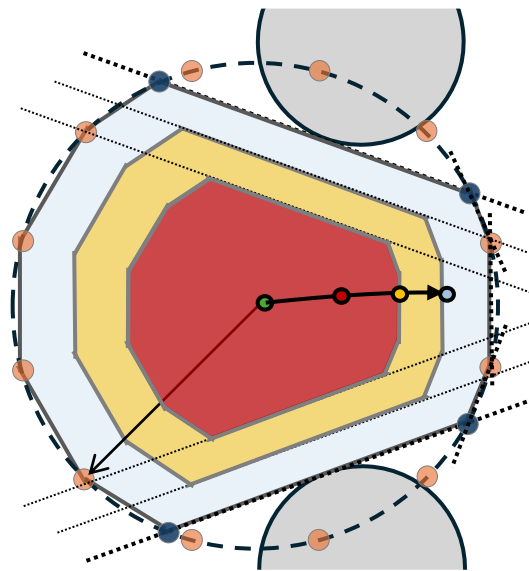
MPPI-DCBF (planner) demonstration
