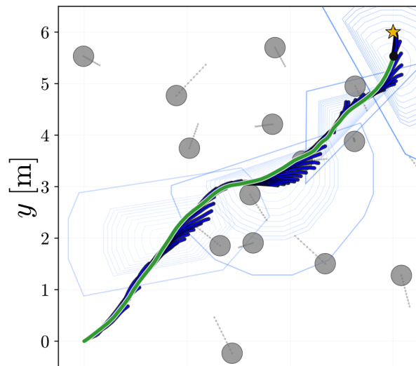
MPPI-DCBF (sparse, slow)
