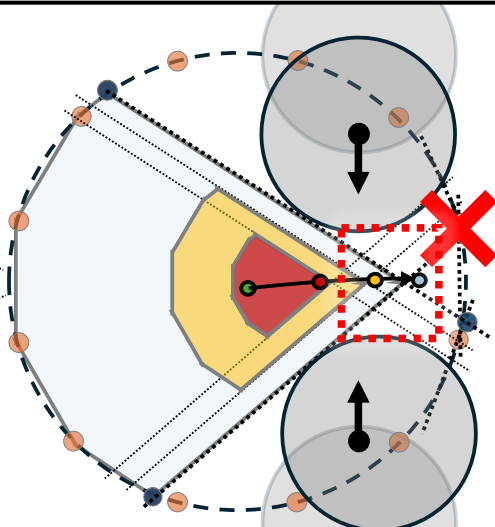
Collision-free action rejected by DCBF
