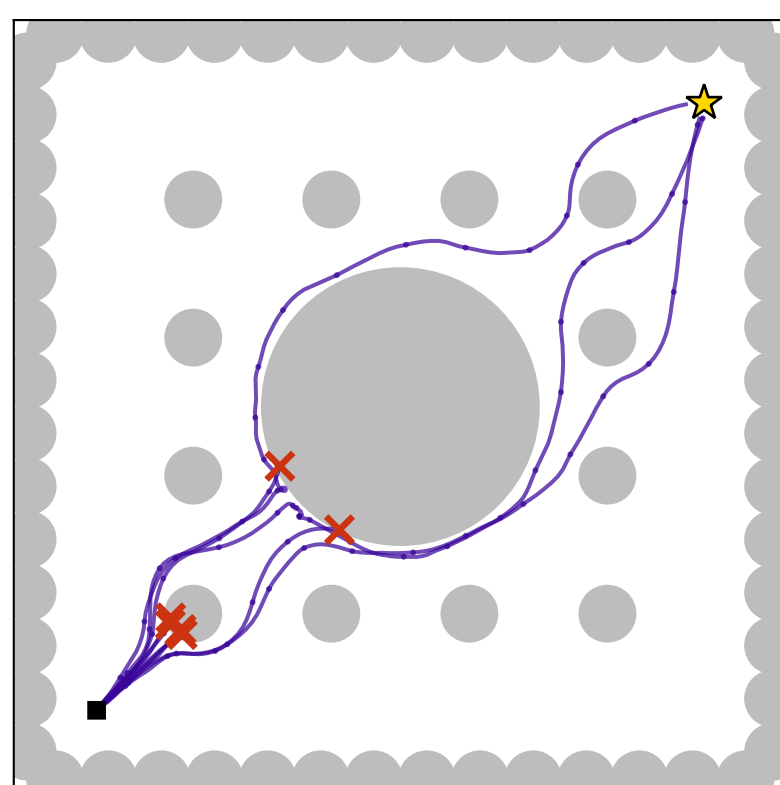
Out of distribution CFM-MPPI* ( w_s = 1.0 )
