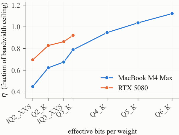
Qwen3.8-27B: efficiency rises with bit width
