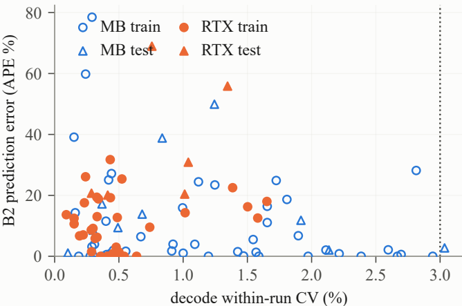
(a) No obvious pooled CV--residual association ( \rho = -0.09 , n=99 )
