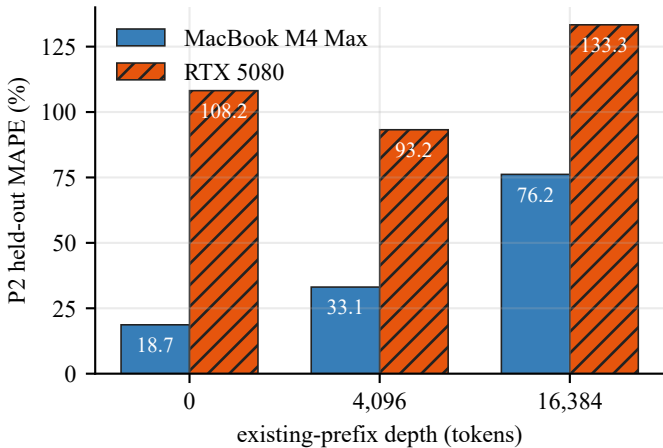
(b) Prefill error is host dependent
