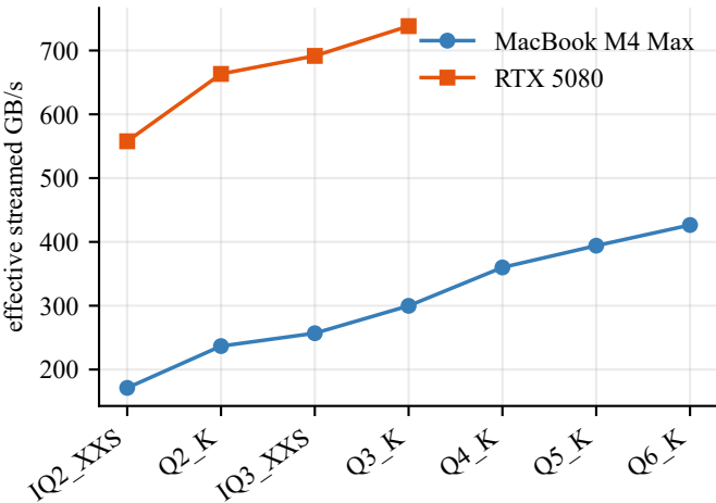
(a) Cross-system Qwen3.8-27B ladder
