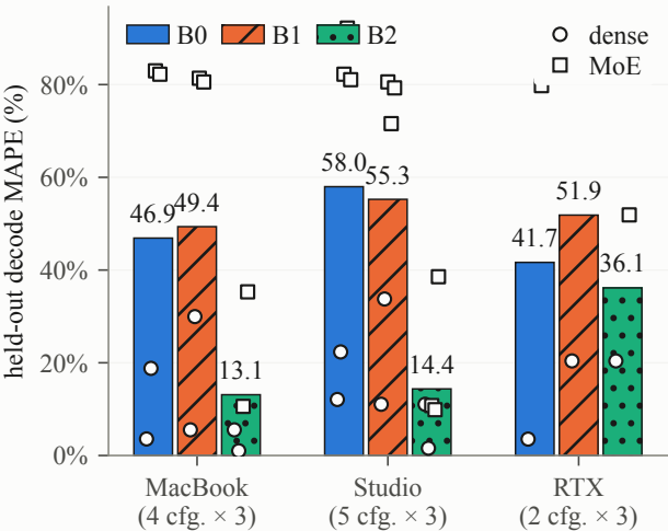
(a) Active-parameter ablation
