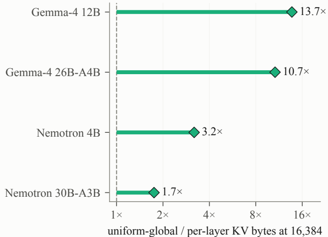
(b) Metadata-aware KV correction
