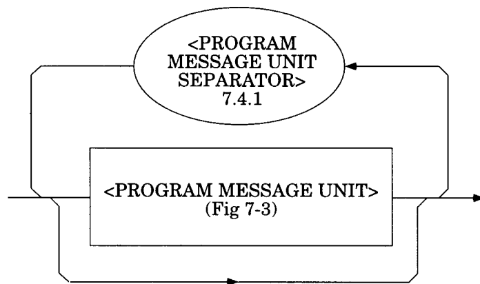
Figure 7-2—&lt;PROGRAM MESSAGE&gt; Functional Element Syntax
