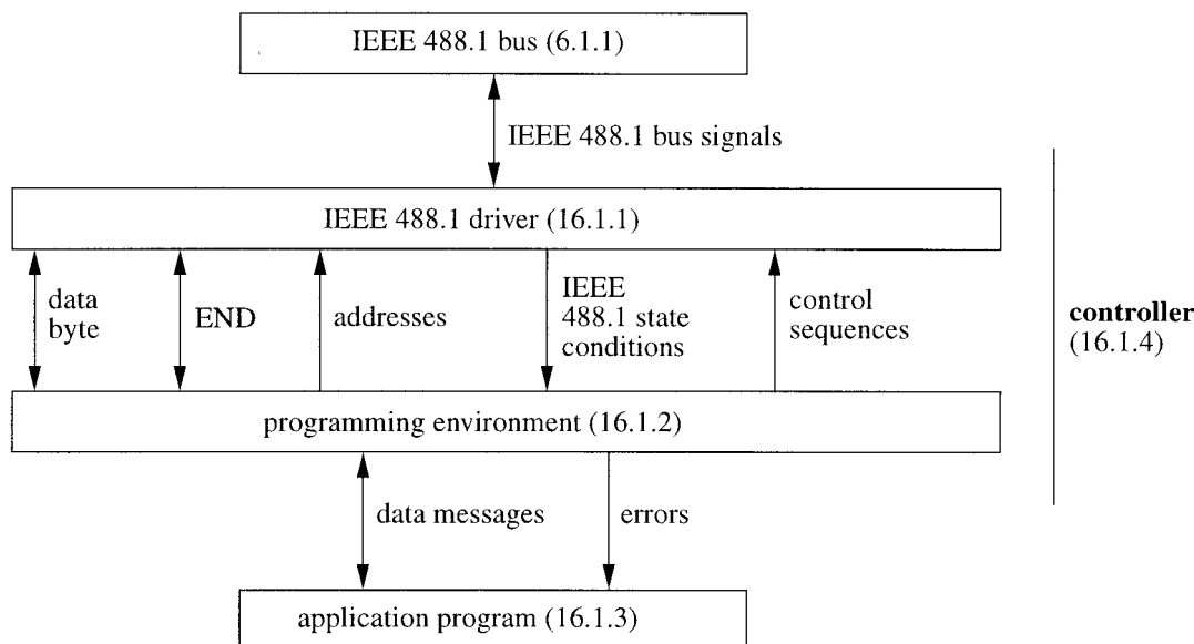
Figure 16-1—Controller Model
