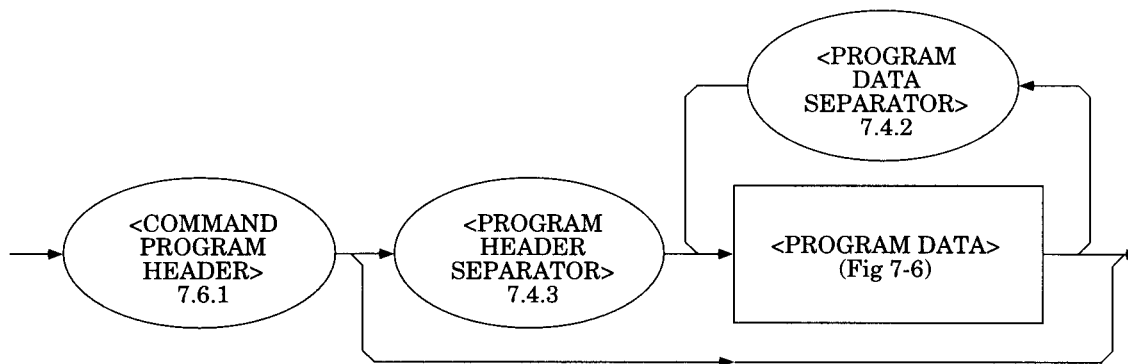
Figure 7-4—&lt;COMMAND MESSAGE UNIT&gt; Functional Element Syntax
