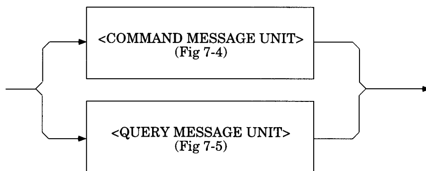
Figure 7-3—&lt;PROGRAM MESSAGE UNIT&gt; Functional Element Syntax
