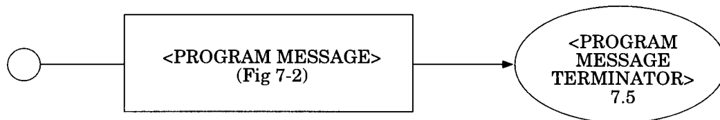
Figure 7-1 — <TERMINATED PROGRAM MESSAGE> Functional Element Syntax
