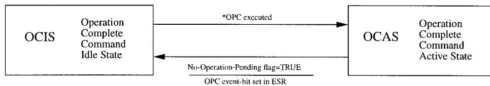
Figure 12-4—Operation Complete Command Diagram
