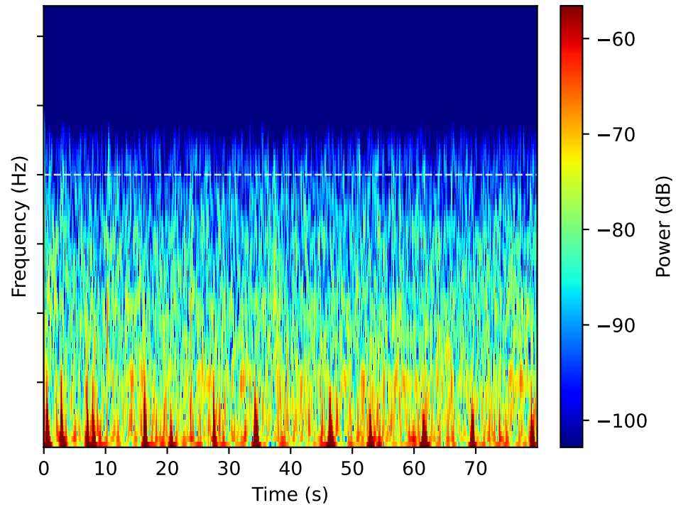
(b) Filtered (0.5-40 Hz) — Fp1
