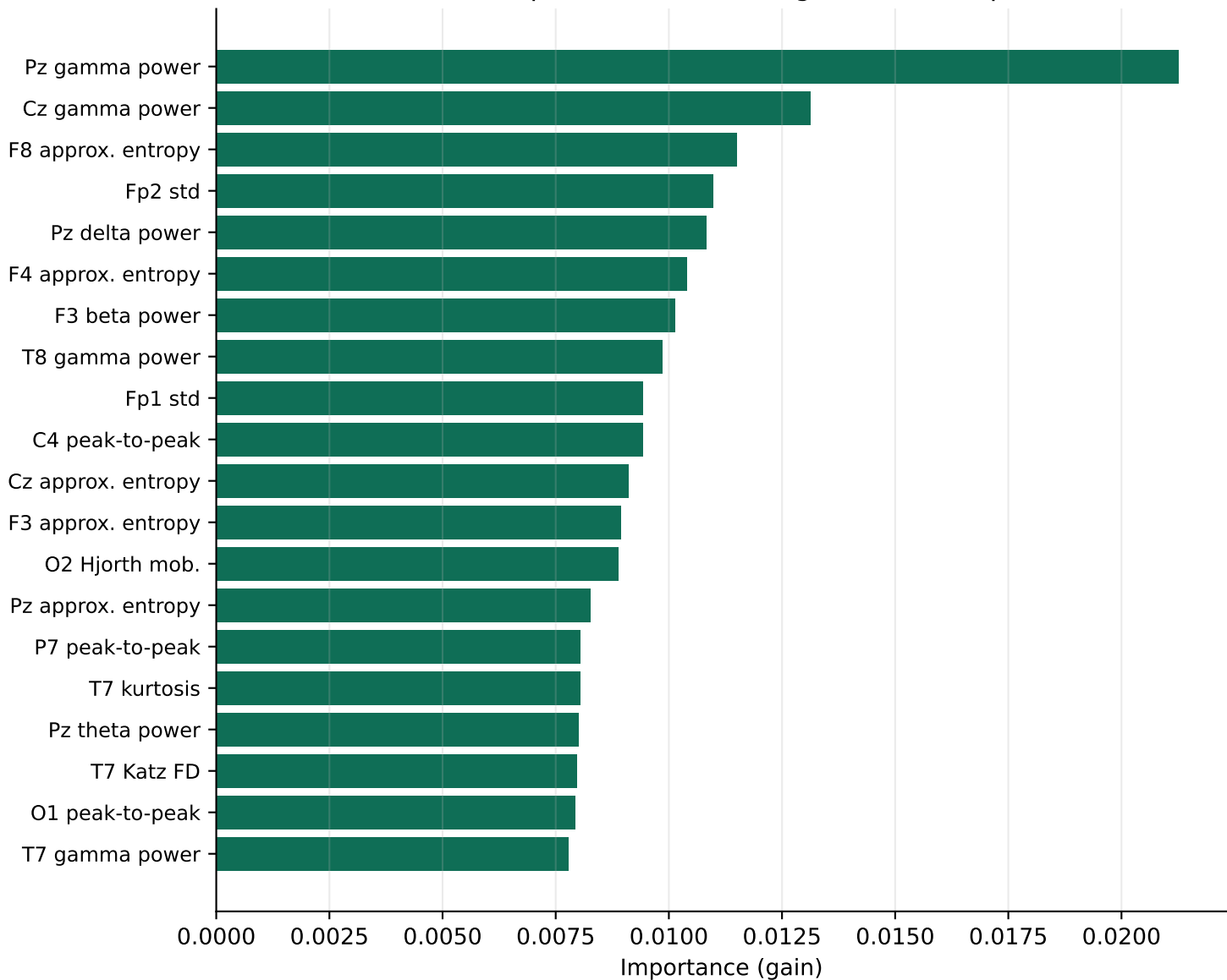
Feature importance (XGBoost gain) — descriptive
