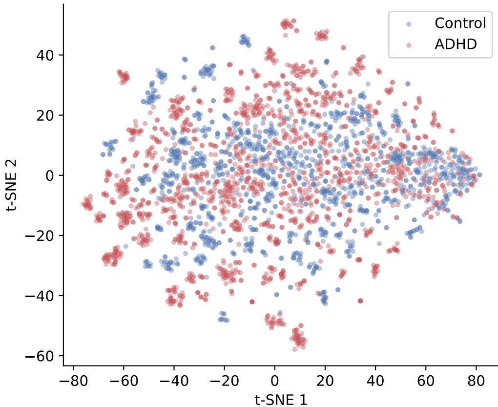
t-SNE projection of epoch features
