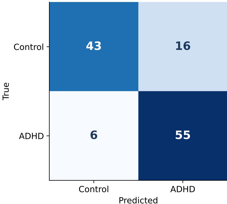
Confusion matrix - XGBoost (LOSO)
