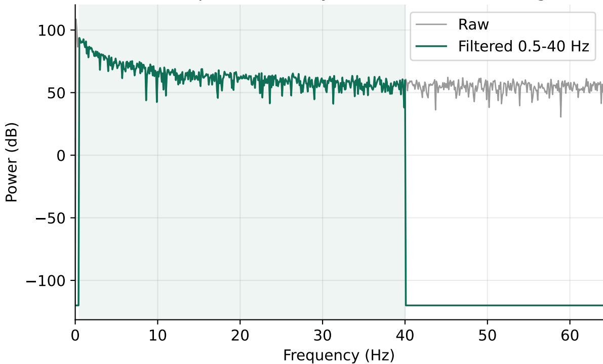
Power spectral density: before vs after filtering
