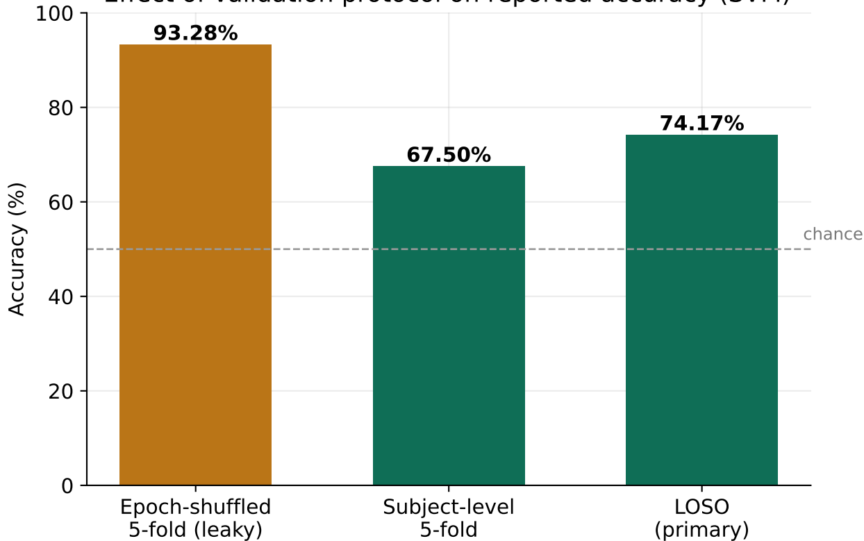
Effect of validation protocol on reported accuracy (SVM)
