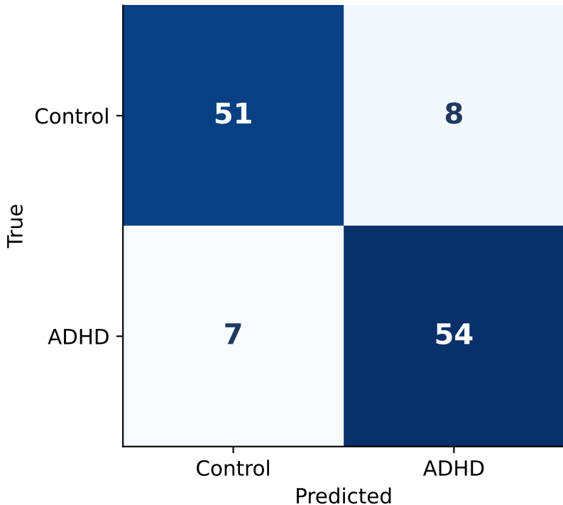
Confusion matrix - SVM (LOSO)
