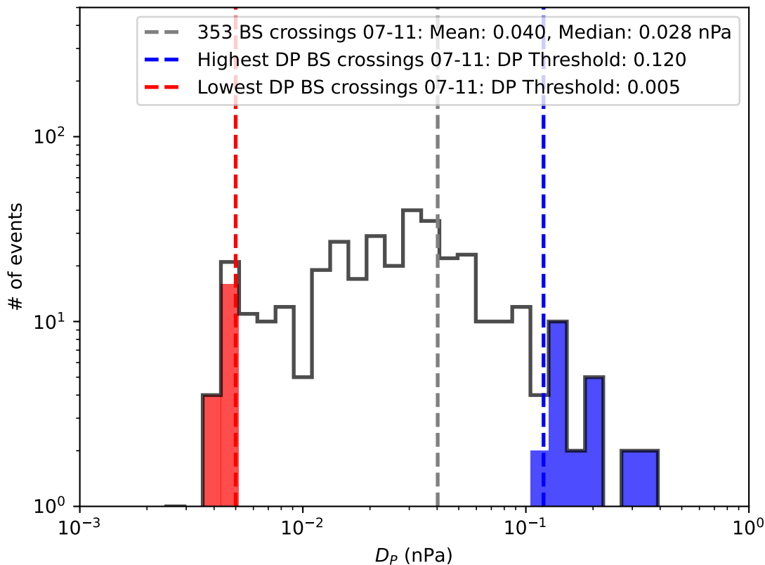
Inferred D_p distribution (BS crossings and LFEs within 50 hours)
