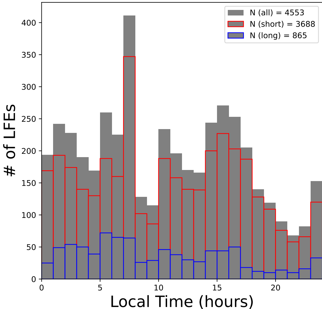
Local Time Distribution of LFES
