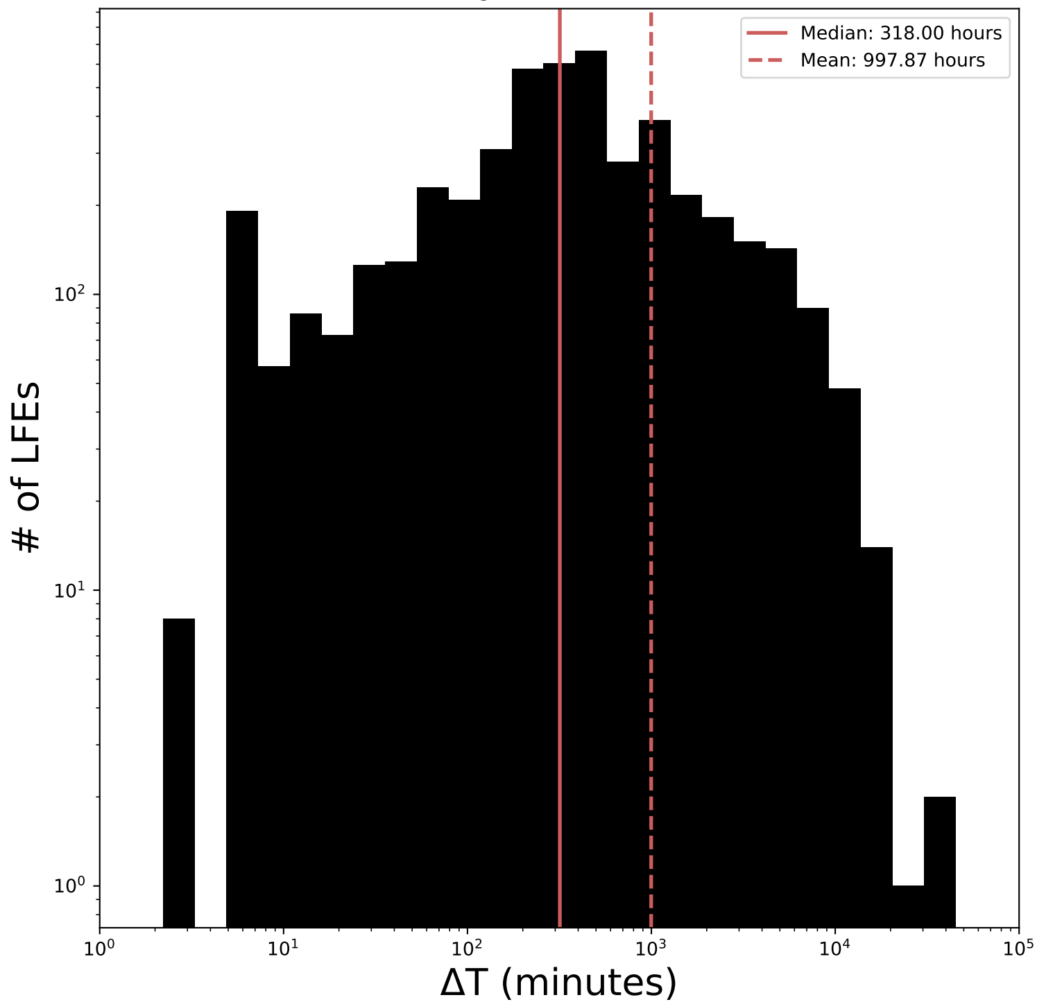
Histogram of LFE \Delta T (all)
