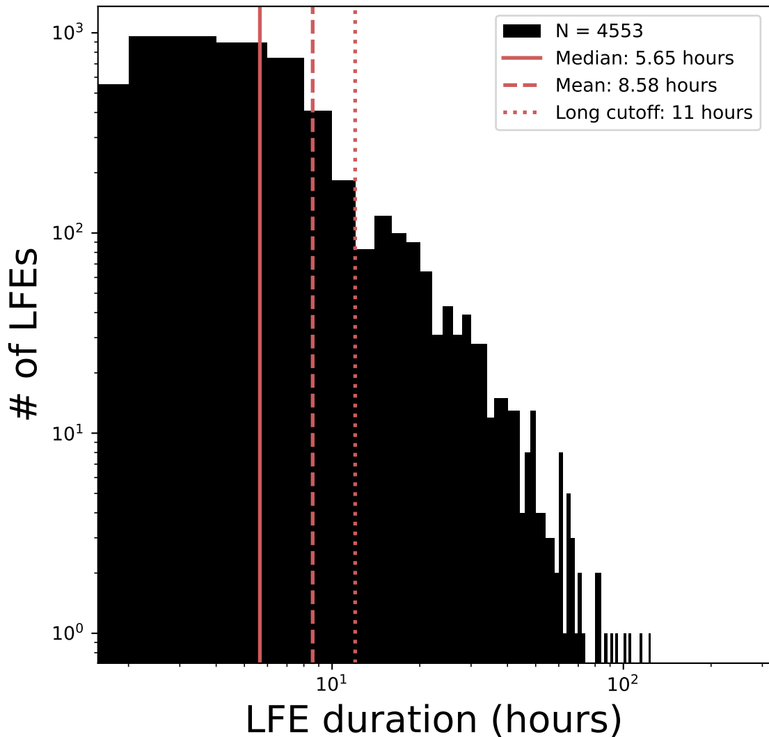
Histogram of LFE duration (Joined List)
