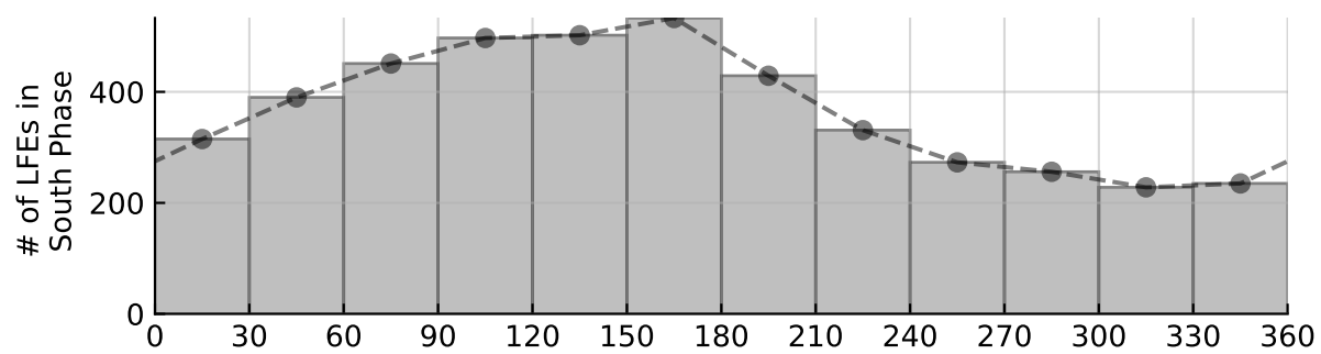
LFE Phase Distribution All: N = 4440
