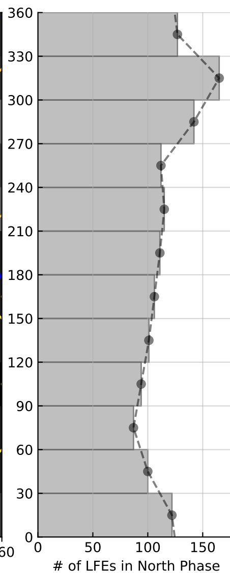
LFE Phase Distribution All, Dawn 03-09: N = 1382
