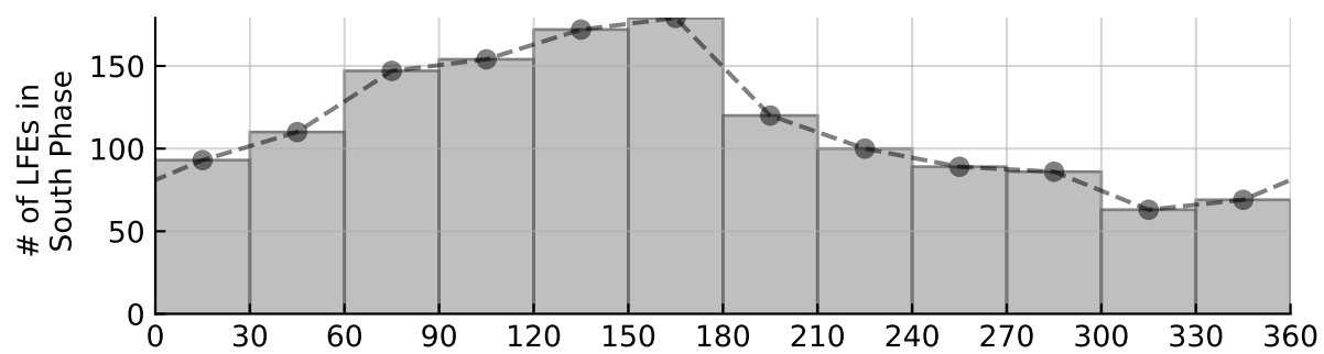
LFE Phase Distribution All, Dawn 03-09: N = 1382
