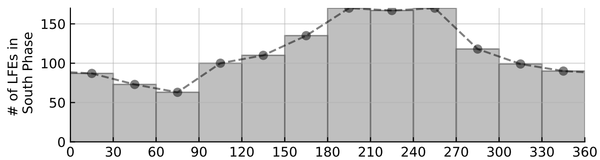
LFE Phase Distribution (Local) All, Dawn 03-09: N = 1382
