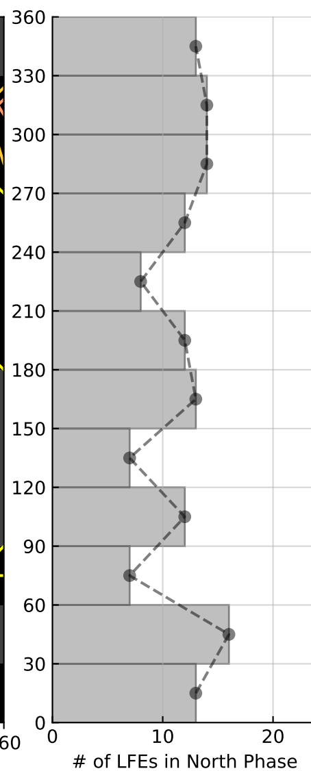
LFE Phase Distribution Long (> 11 hr), Dusk 15-21: N = 141
