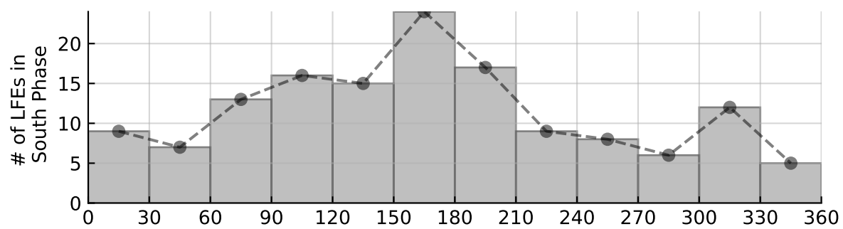
LFE Phase Distribution Long (> 11 hr), Dusk 15-21: N = 141
