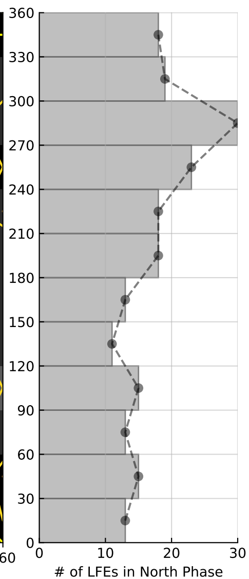
LFE Phase Distribution Long (> 11 hr), Noon 09-15: N = 206
