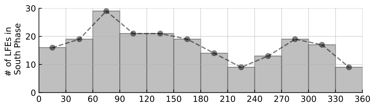
LFE Phase Distribution Long (> 11 hr), Noon 09-15: N = 206
