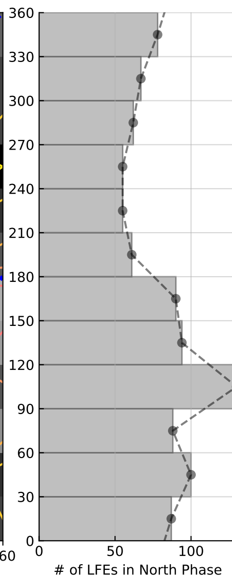
LFE Phase Distribution (Local) All, Midnight 21-03: N = 967
