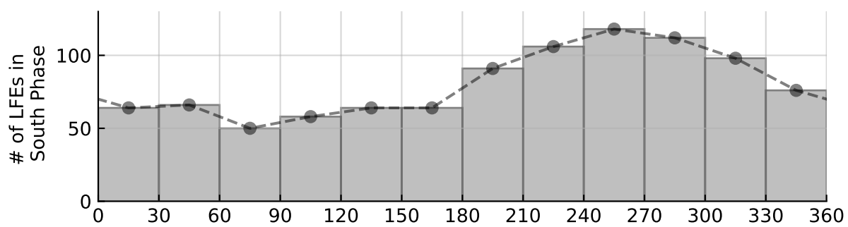
LFE Phase Distribution (Local) All, Midnight 21-03: N = 967
