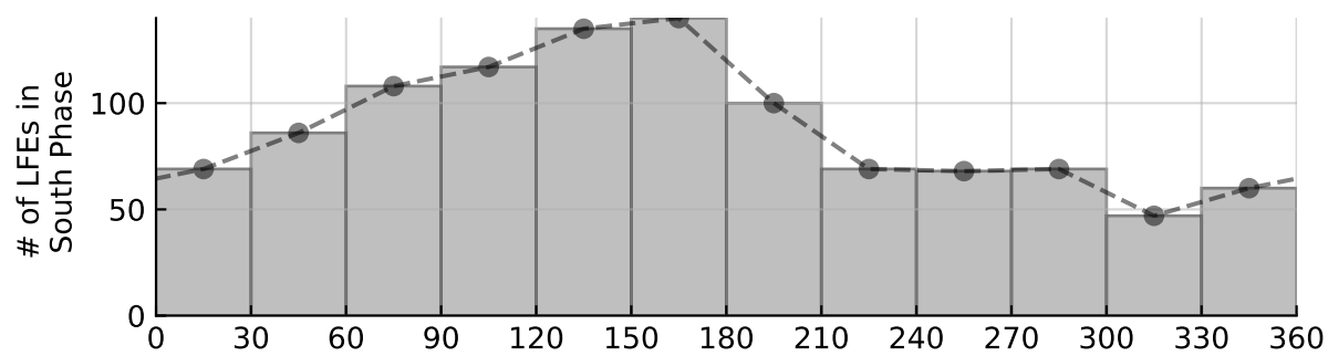
LFE Phase Distribution Short (< 11 hr), Dawn 3-9: N = 1068
