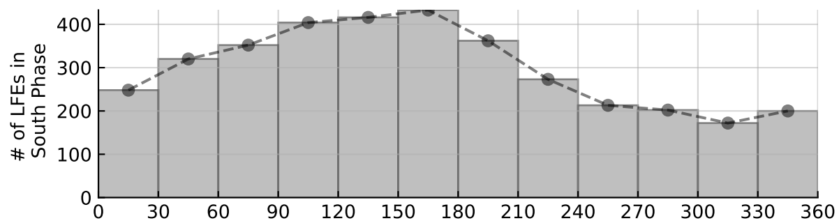
LFE Phase Distribution Short (< 11 hr): N = 3595
