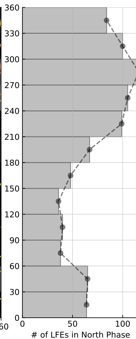
LFE Phase Distribution Short (< 11 hr), Noon 09-15: N = 862
