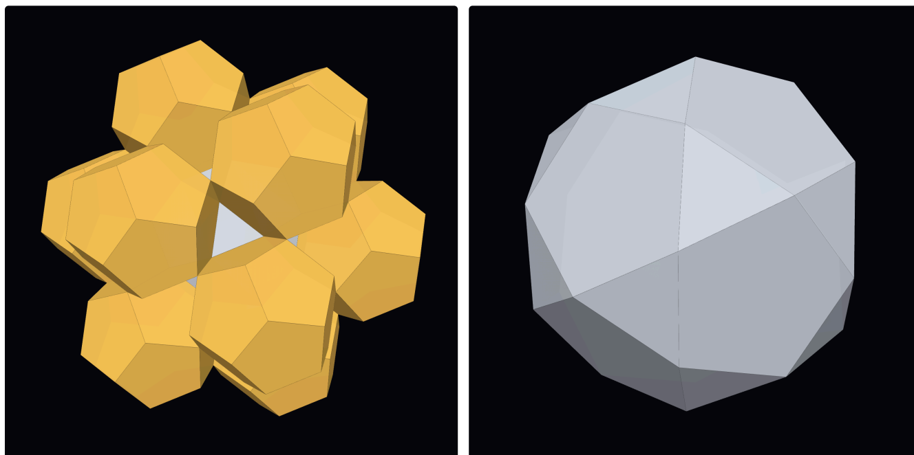
Fig. 4-5. (4) The dodecahedra alone, leaving the 20 three-fold dimples the J63s fill, seen down a three-fold axis. (5) The icosidodecahedron at the centre.
