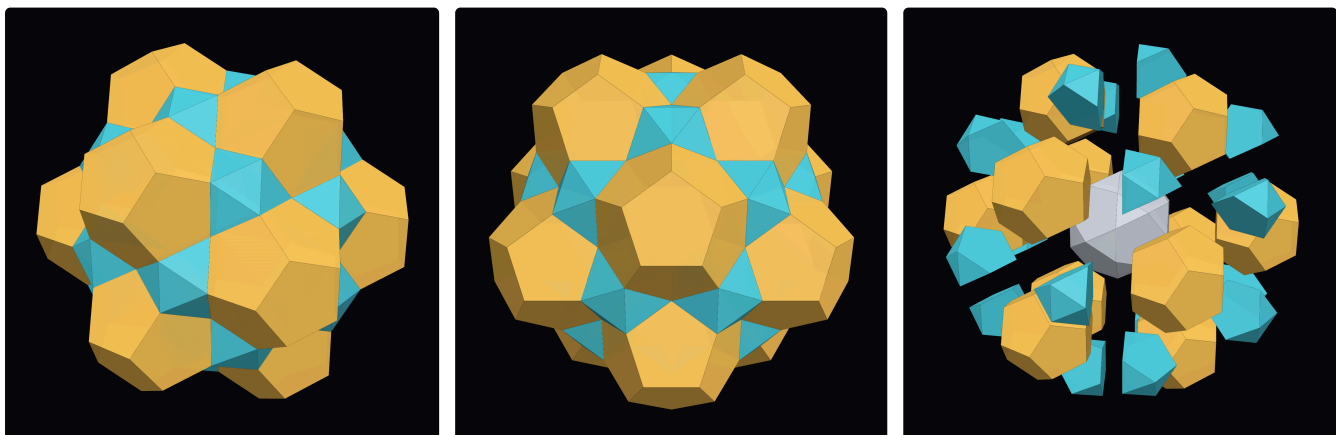
Fig. 1-3. (1) The DICTO-Star: 12 dodecahedra (gold) and 20 tridiminished icosahedra (cyan) on an icosidodecahedron. (2) The same, down a five-fold axis. (3) Pulled apart: the icosidodecahedron (grey) at the centre.
