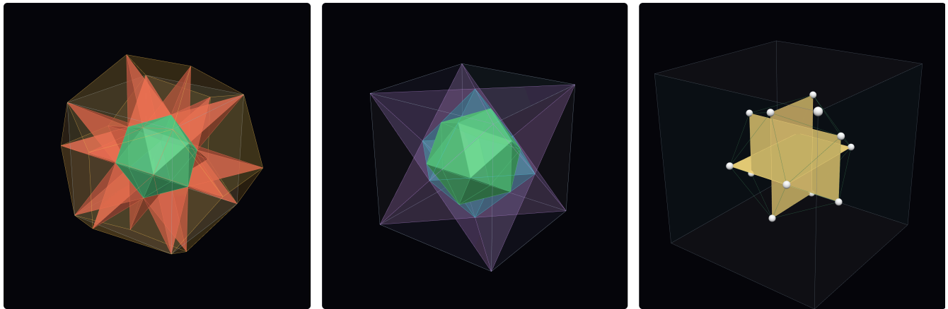
Fig. 1-3. (1) One cell: the cube (grey), Euclid's dodecahedron (gold), Kepler's great stellated dodecahedron (orange) and the icosahedron (green), all on the same 20 + 12 points. (2) Kepler's chain: icosahedron \subset octahedron (cyan) \subset stella octangula (violet) \subset cube. (3) Pacioli's three golden rectangles ( 2/\phi \times 2/\phi^2 ) whose 12 corners are the icosahedron; each is a pair of ridges from the neighbouring cells.
