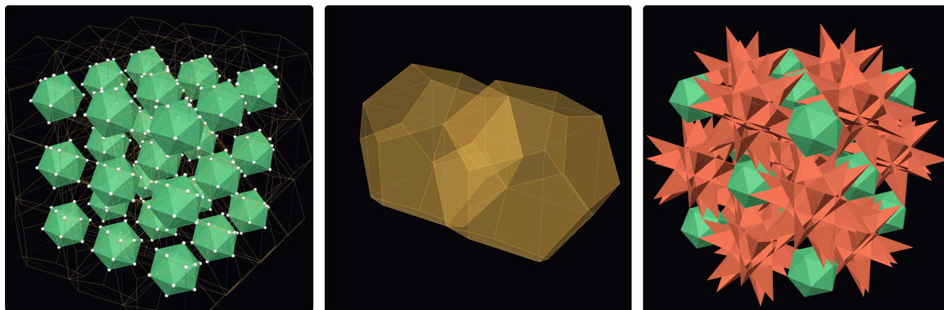
Fig. 4-6. (4) A 3 \times 3 \times 3 block of cells: icosahedra, dodecahedron edges (gold), cube edges and the 13 nodes per cell (white). (5) Two face neighbours: their dodecahedra overlap by exactly two roofs. (6) The EKP network: great stellated dodecahedra on even cells, icosahedra on odd cells, meeting at corners only.
