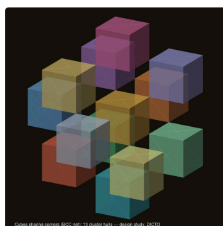
Fig. 4-7. (4) Cuboctahedra sharing corners (FCC). (5) Cubes sharing corners (BCC). (6) Octahedra sharing corners (simple cubic, the perovskite net). (7) The rhombic-dodecahedral hull in the Stella-Jewel Lattice, its corner stellas in violet.
