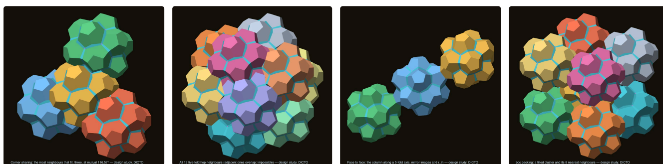
Fig. 8-11. (8) The most corner-sharing neighbours that fit: three, at mutual 116.57^\circ . (9) All 12 five-fold neighbours at once: adjacent ones overlap. (10) The face-to-face column along a five-fold axis. (11) The densest stacking, bcc.
