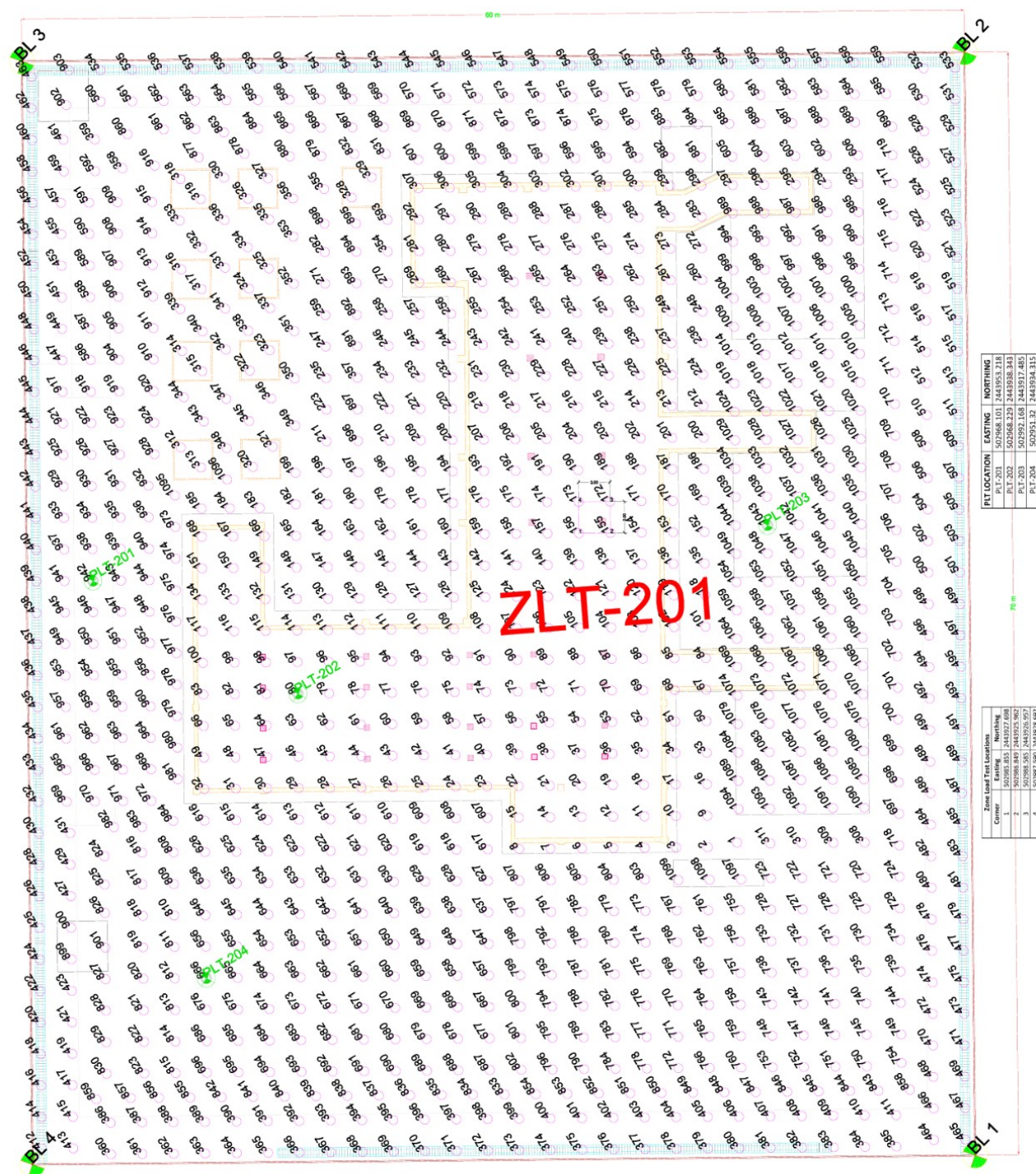
Figure 5-8. As-built layout of the rigid-inclusion works: the 1,075 controlled modulus columns within the 4,200 m 2 improved-ground boundary, the building and equipment foundation footprints, and the plate-load-test (PLT-201 to 204) and zone-load-test (ZLT-201) locations. reproduced from the project as-built drawing (anonymized).
