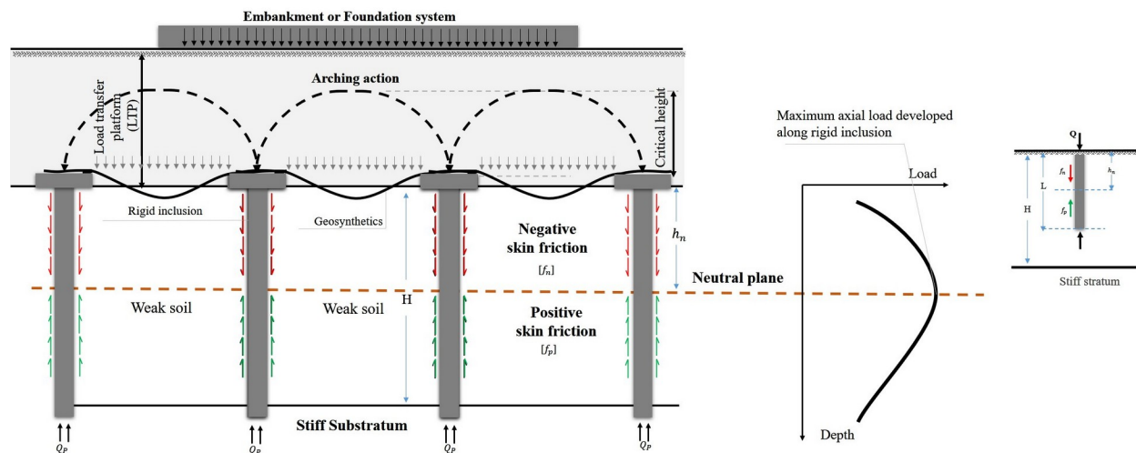
Figure 3-9. Load transfer in a rigid-inclusion system. Soil arching over the critical height concentrates the embankment or foundation load onto the inclusion heads through the load-transfer platform and its geosynthetic; below, negative (downdrag) skin friction ( f_n ) develops above the neutral plane and positive skin friction ( f_p ) below it, so that the axial load in the inclusion is greatest at the neutral plane before being shed to the base ( Q_p ). The inset shows the corresponding axial-load-versus-depth distribution. provided by the project team.
