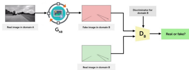
Figure: ICGA architecture for road-surface crack detection.
