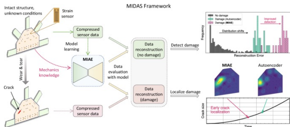
Figure: Mechanics-informed damage-detection and localization framework.
