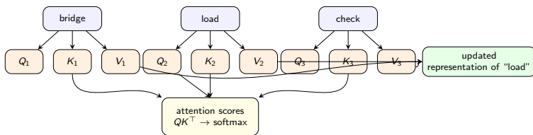
Figure: Self-attention: the token “load” compares against the full context instead of relying only on sequential memory.
