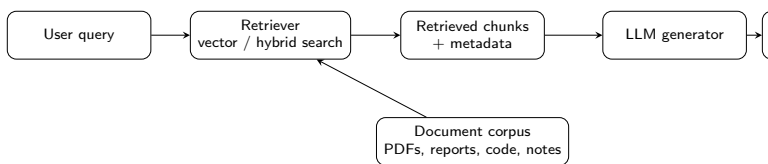
Figure: A practical RAG pipeline for engineering knowledge work.
