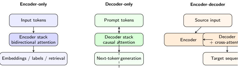
Figure: Three mainstream transformer families.
