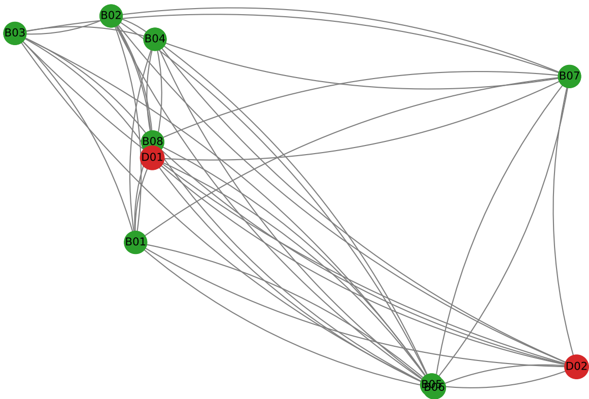
Bridge Subgraph
