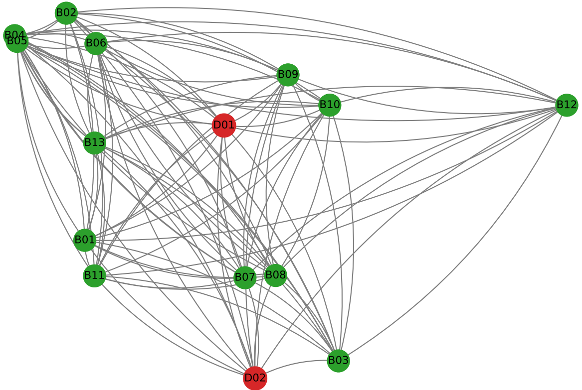
Bridge Subgraph
