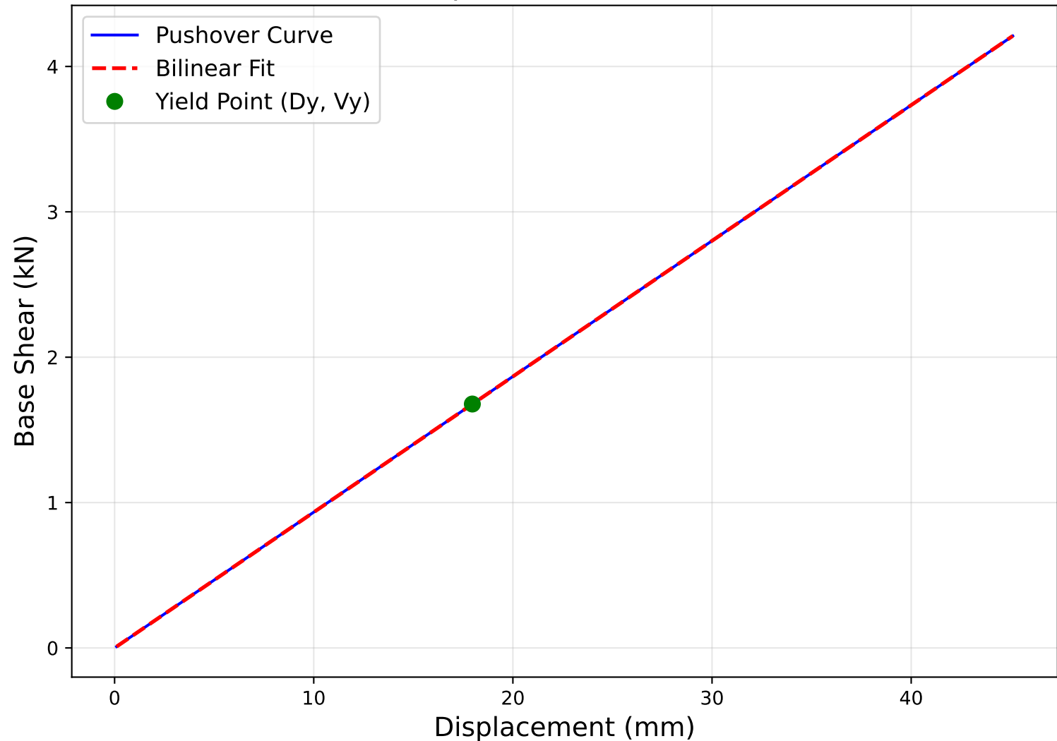
Pushover Curve - Displacement vs Base Shear (Missouri)
