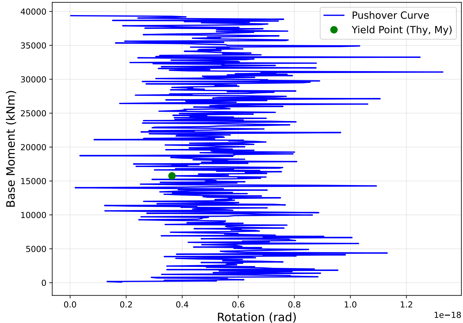
Pushover Curve - Rotation vs Base Moment (Missouri)
