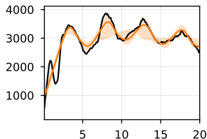
Cell 93 (fold 3)
