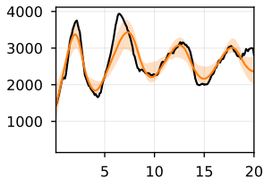
Cell 51 (fold 1)
