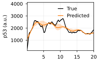
Cell 0 (fold 0)
