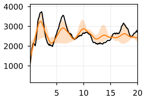
Cell 35 (fold 4)
