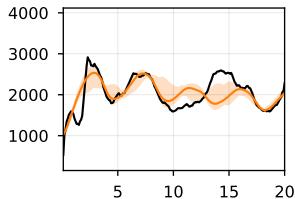
Cell 100 (fold 2)
