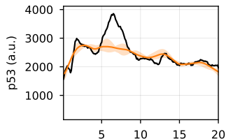
Cell 58 (fold 3)
