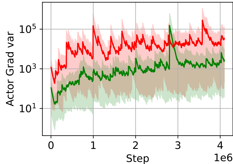
SHAC vs. SHACTDFixed
