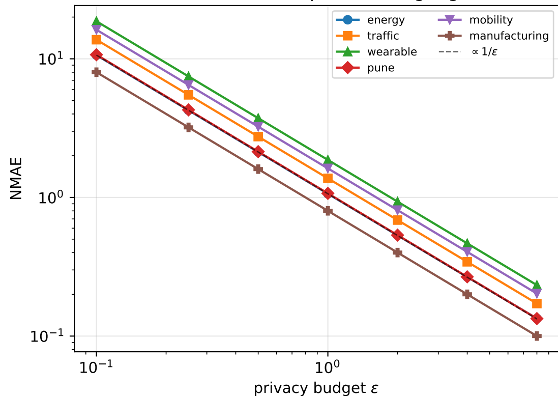
NMAE \propto 1/\epsilon (slope -1 on log-log)
