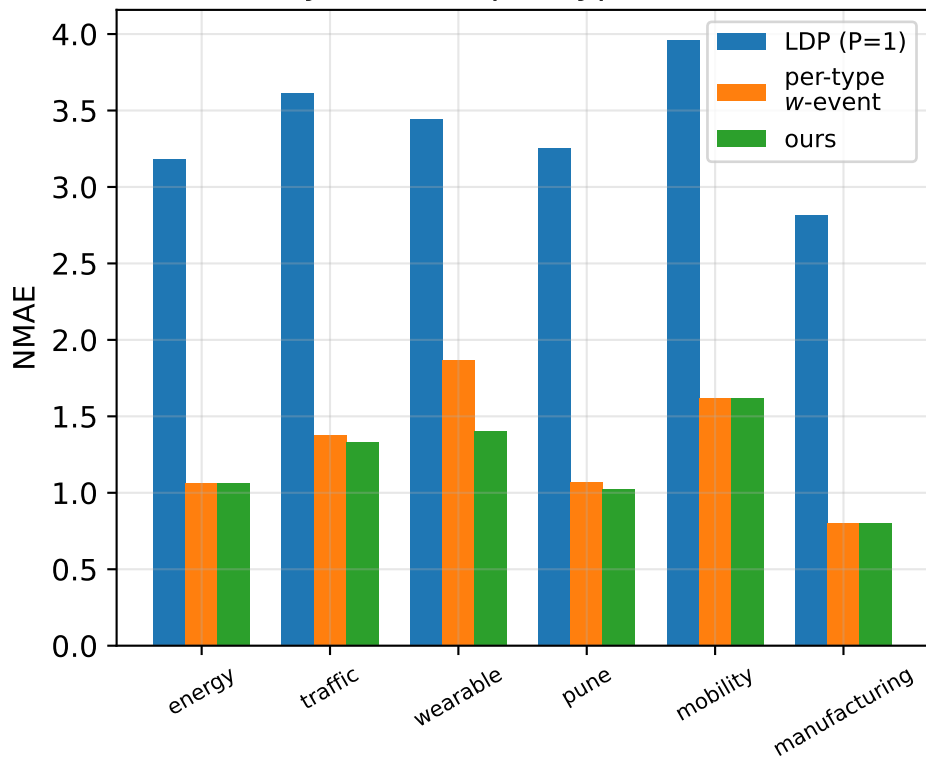
(a) Utility: ours \approx per-type, both \ll LDP
