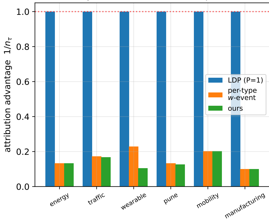
(b) Privacy: ours \ll LDP's full exposure (=1)
